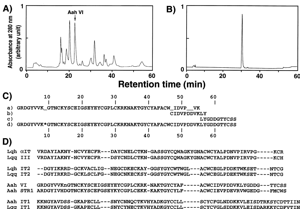
Fig. 1. Purification steps, and sequence determination and comparison. A: CM MemSep chromatography of the RIT fraction from recycling chromatography. B: RP-HPLC of the Aah VI fraction from CM MemSep. Details are given in Section 2. C: Amino acid sequencing of Aah VI. (a) Results of Edman degradation of RPE-Aah VI (—: unidentified residues); (b) chymotryptic peptide; (c) tryptic peptide; (d) complete sequence of Aah VI as deduced from a–c. The star indicates the glycosylated Asn residue. D: Sequence comparison with alignment of the half-cystine residues. The sequences were taken from references [4,16–20]. n: glycosylated asparagine residue.
